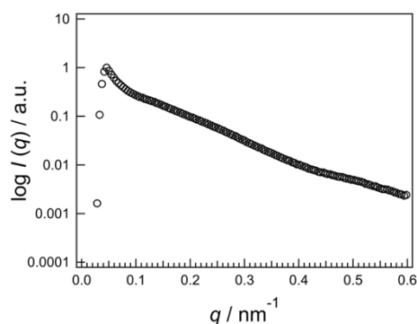
Figure 2. SAXS profiles of the ethylene-anisylpropylene multi-block copolymer.
