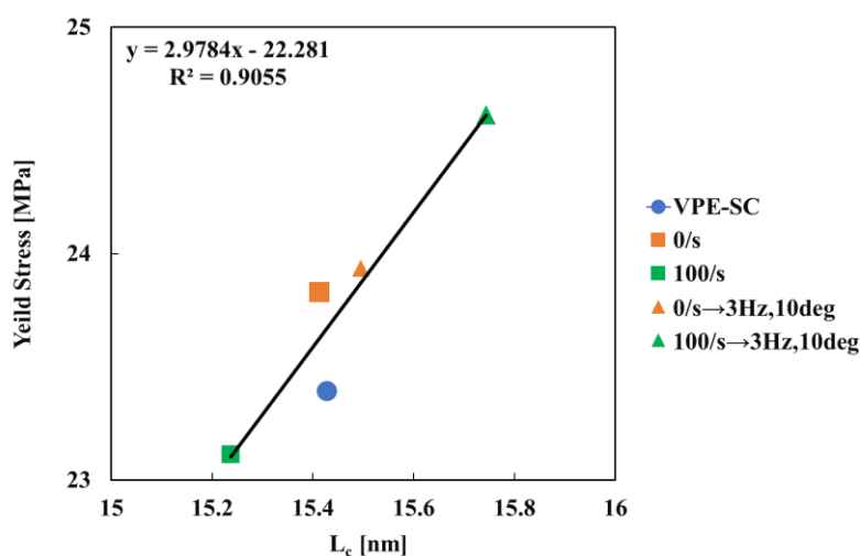
Fig. 1 Relationship between thickness of crystalline layer ( L_c ) and yield stress of virgin HDPE thin film (VPE-SC) and shear-treated HDPE with various shear treatment conditions.
