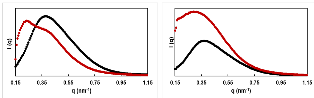
Fig. 1 SAXS profile of V-LDPE (Black line) and 24h-100C (Red line) compared between two grades of LDPE thin film (J2522; left-side graph, and F522N; right-side graph).
