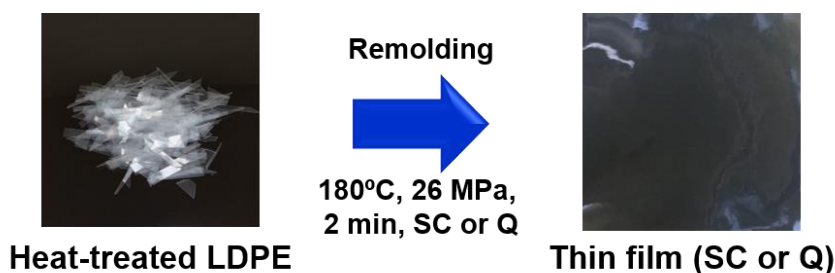
Fig. 1 Fabrication of thin film (100 \mu\text{m} of thickness) by hot compression
