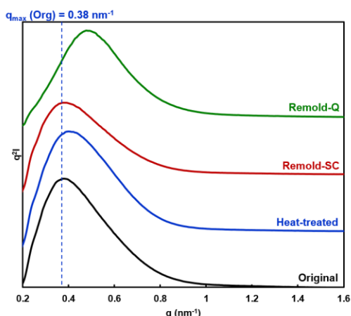
Fig. 2 SAXS profile of LDPE original, LDPE after heat treatment (Heat-treated), Remolding LDPE with slow cooling (Remold-SC), and Remolding LDPE with quench cooling (Remold-Q).
